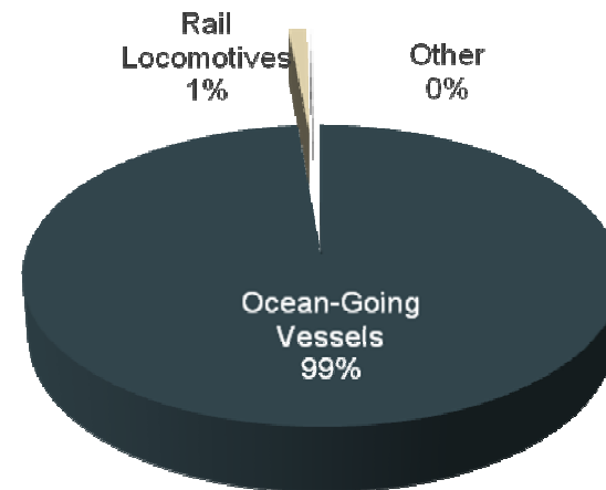
SOx
