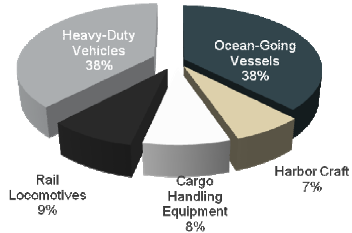
SOx
