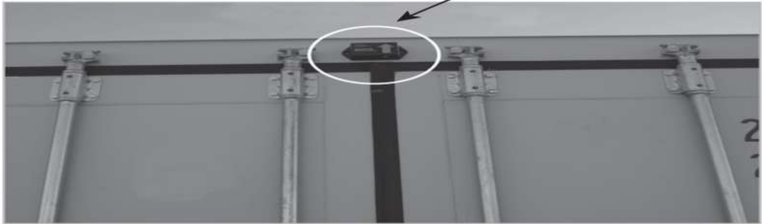
iControl's MATTS tag mounted on the outside of a container, above container doors.
