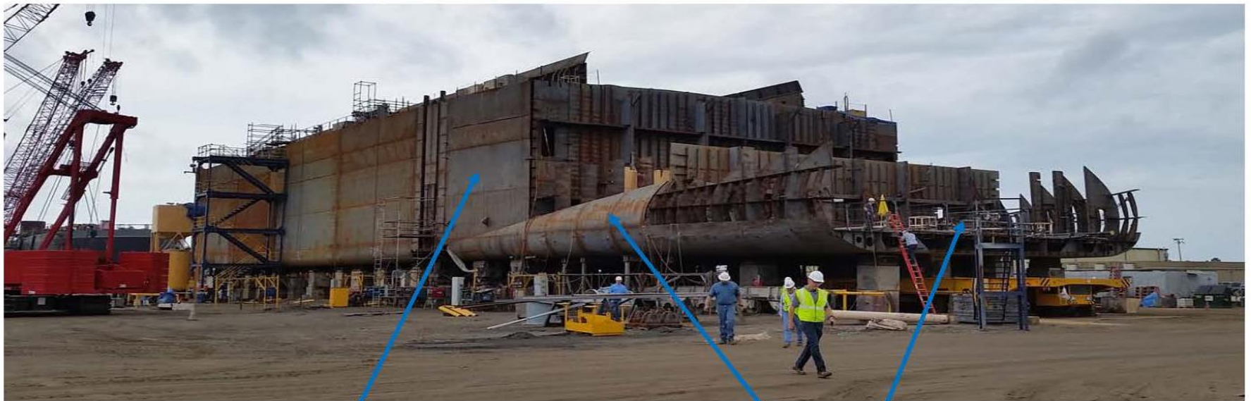
Starboard Bow – Hopper begins at Module 4. Module 2a and 3 (foremost sections) are pump and engine compartments.
